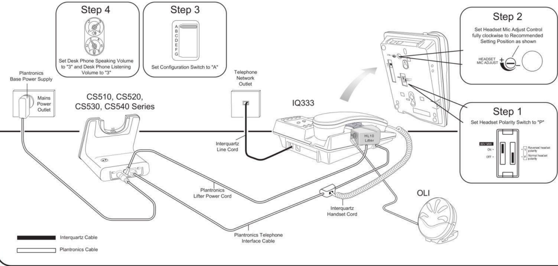
Figure 1 - CS510, CS520, CS530, CS540 Series & OLI Connection Diagram for IQ333
