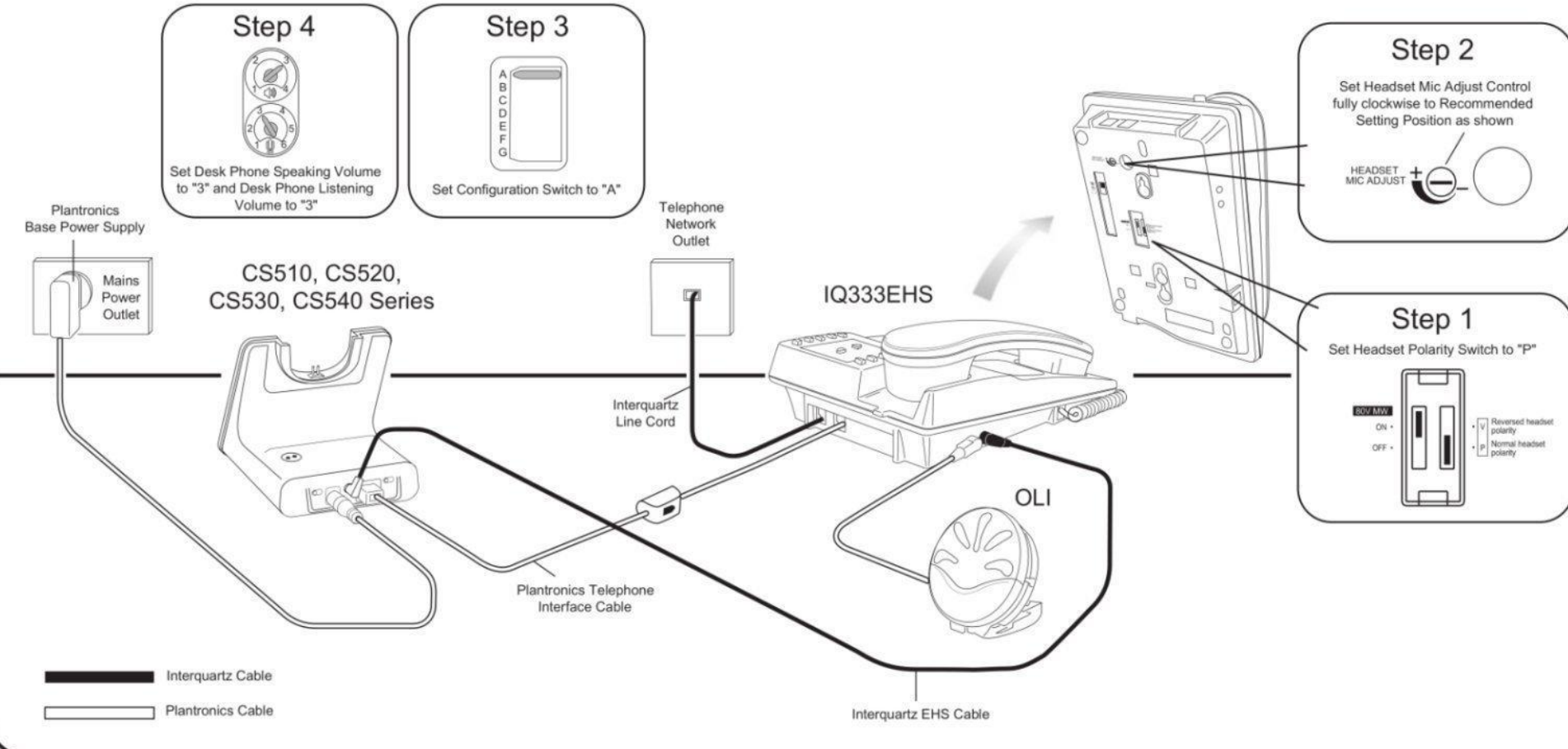
Figure 2 - CS510, CS520, CS530, CS540 Series & OLI Connection Diagram for IQ333EHS
